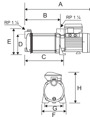
Dimensions [mm]
